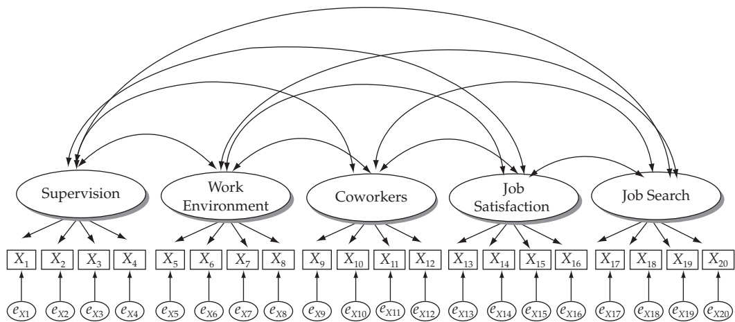
FIGURE 9 A Path Diagram Showing Hypothesized Measurement Model Specification (CFA Model)
