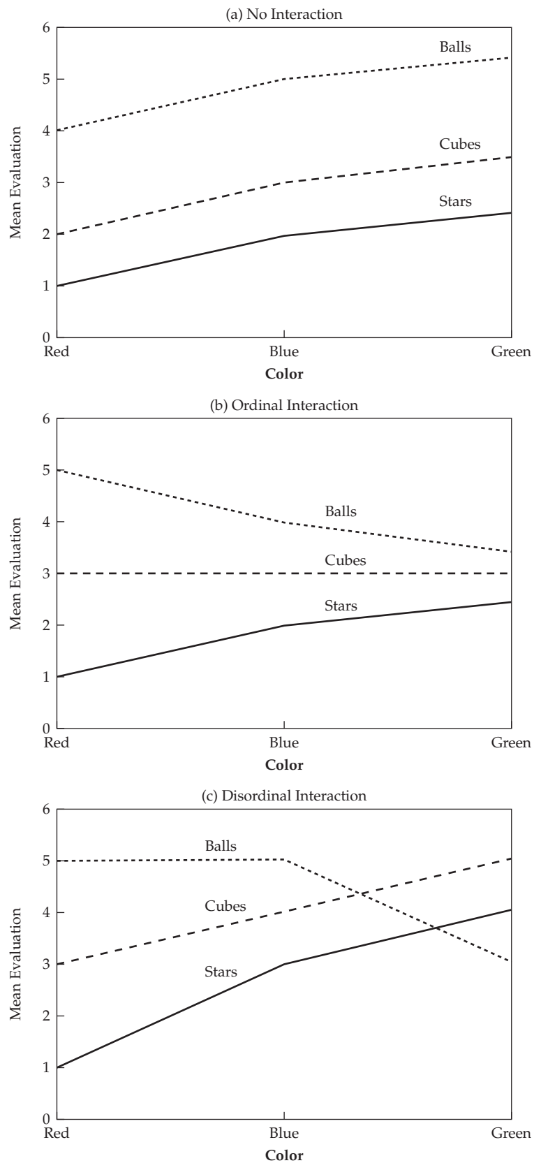
FIGURE 5 Interaction Effects in Factorial Designs
