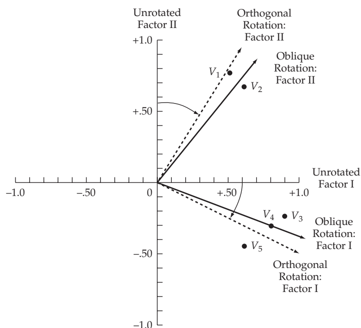
FIGURE 8 Oblique Factor Rotation
